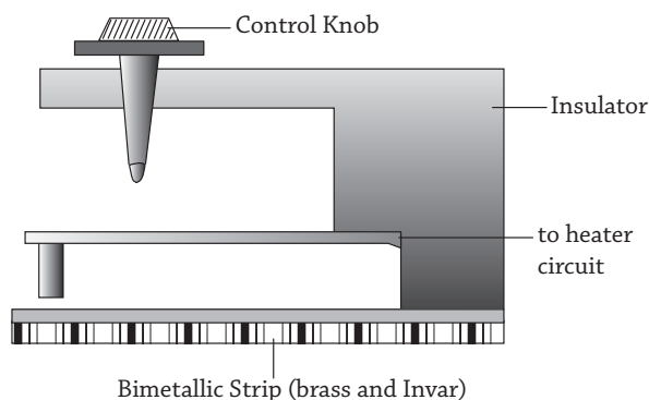
Fig 14.19 : A thermostat
