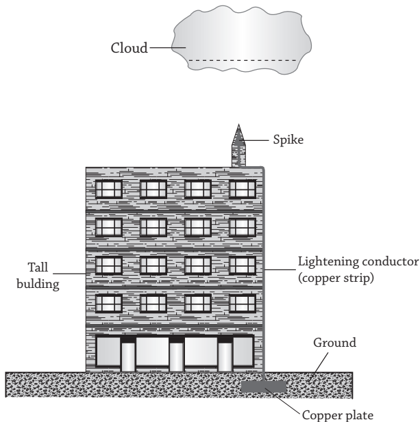
Fig 16.16 : Lightning conductor
