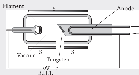
Figure 22.11 : A Modern X-ray tube
