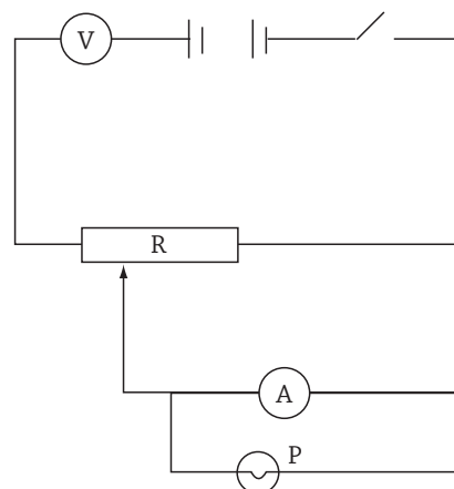
Fig 17.1: Electric circuit
