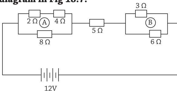
Fig 18.7 : A Circuit diagram
