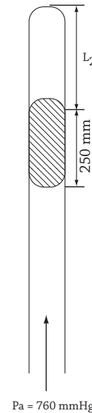
Fig 15.6 : A tube with open end down
