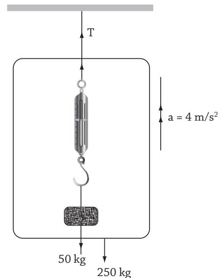
Fig 11.22 : Spring balance in a lift
