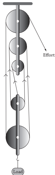
Fig 10.13 : Block and tackle pulley
