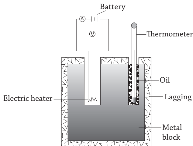
Fig 15.14 : Specific heat capacity by electrical method
