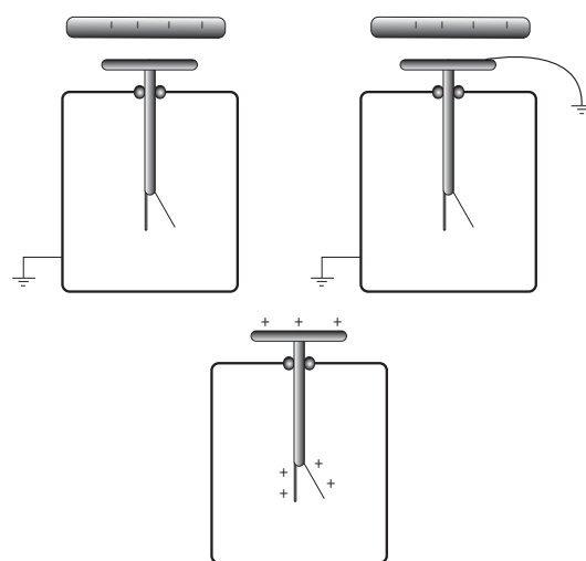
Fig 16.10 : Charging gold leaf electroscope by induction
