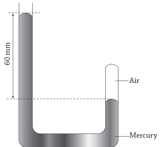
Fig 8.10 : Closed end manometer
