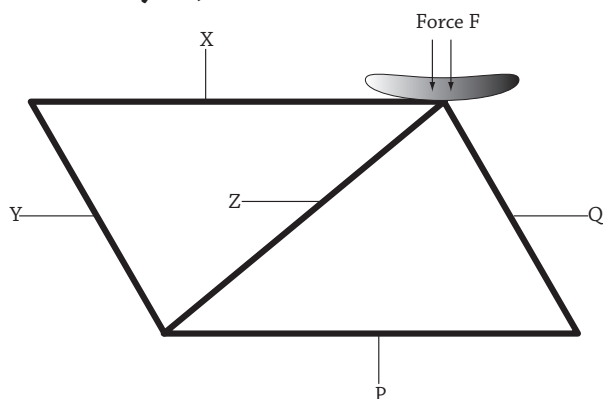
Fig. 5.3 : Type of forces on bicycle frame
