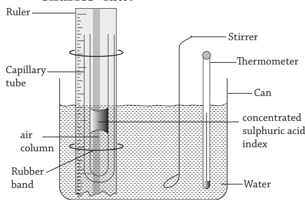
Fig 15.7 : Verifying Charles' law
