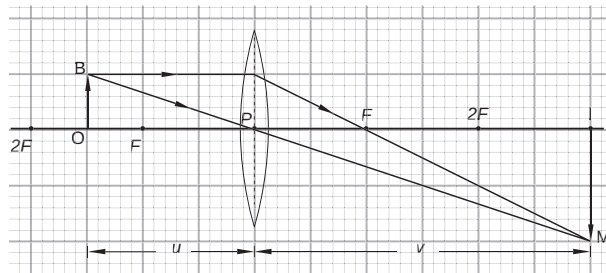
Fig 12.39 : Image formed on convex lens
