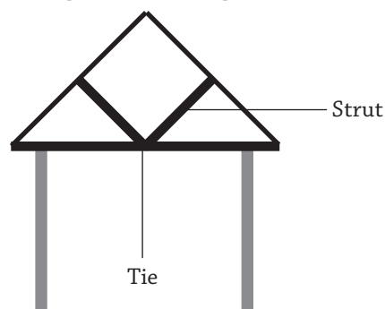
Fig 5.4 : Roof structure
