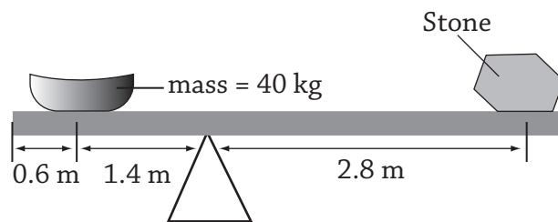
Fig. 3.4: Beam balance
