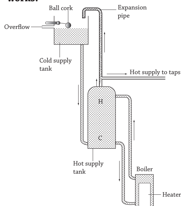
Fig 14.11 : Hot water supply boiler
