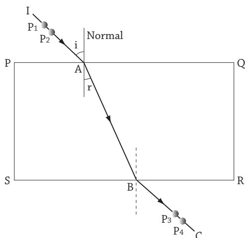
Fig 12.14 : Determining refractive index of a glass block
