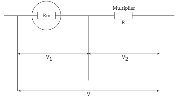
Fig 18.13 : Moving coil galvanometer
