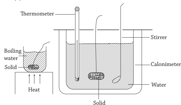
Fig 15.13 : Determining specific heat capacity of a solid
