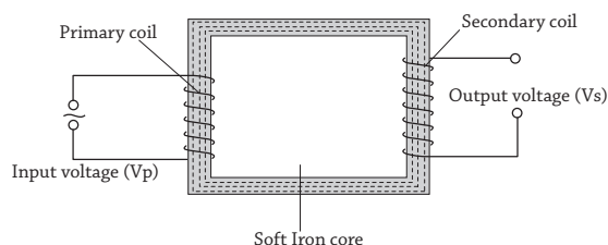
Fig 21.6 : A transformer
