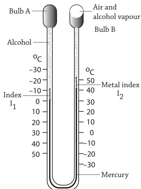
Fig 14.2 : A Six's minimum - maximum thermometer
