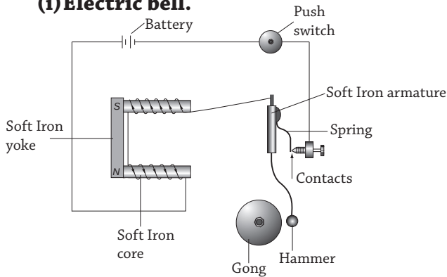
Fig 20.6 : An electric bell
