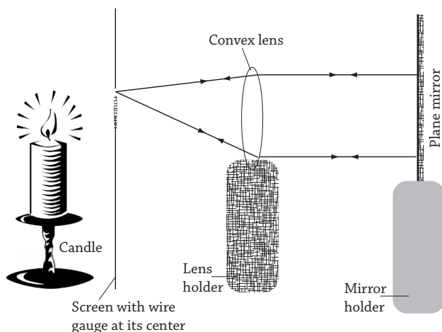
Fig 12.24 : Determining length of a convex lens
