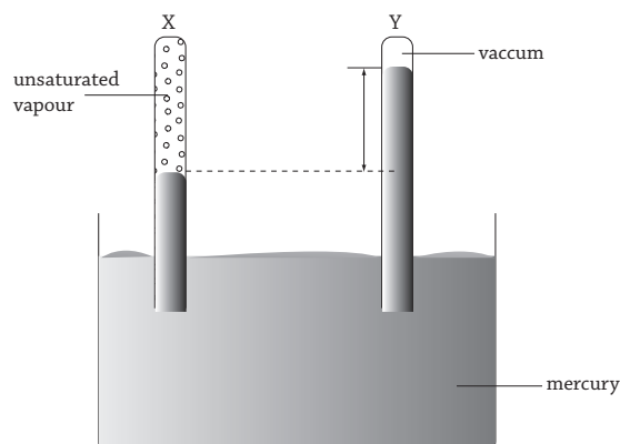
Fig 15.20 : Measuring the vapour pressure of water
