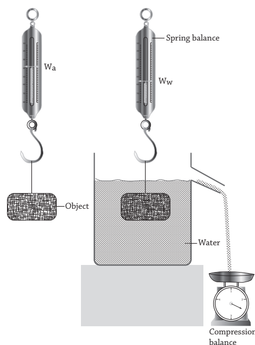
Fig 9.2 : Verification of Archimede's principle
