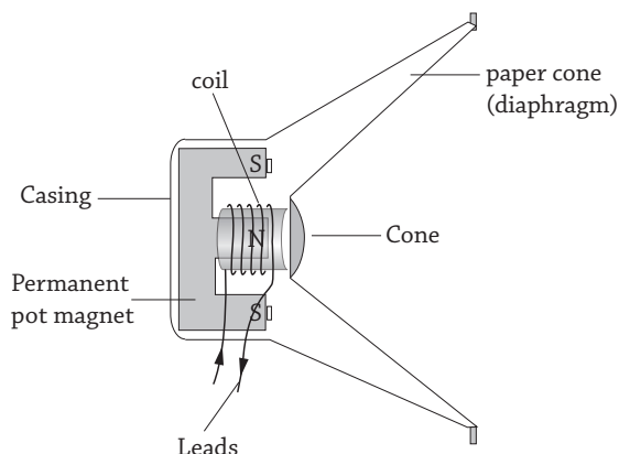
Fig 20.12 : A moving coil loudspeaker
