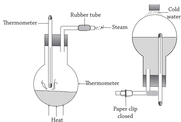
Fig 15.18 : Effect of pressure on boiling point
