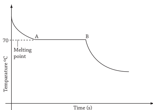
Fig 15.19 : Cooling curve of Ethanamide
