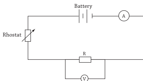
Fig 18.2 : Verification of ohm's law
