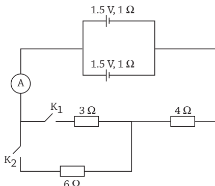
Fig 18.9 : An electric circuit
