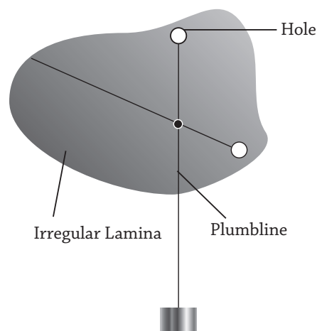
Fig. 3.7 : Centre of gravity of a lamina
