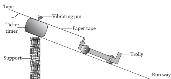
Fig 11.9 : A trolley sliding
