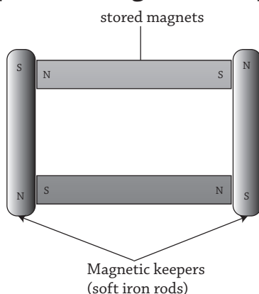
Fig 19.15 : Magnetic keepers
