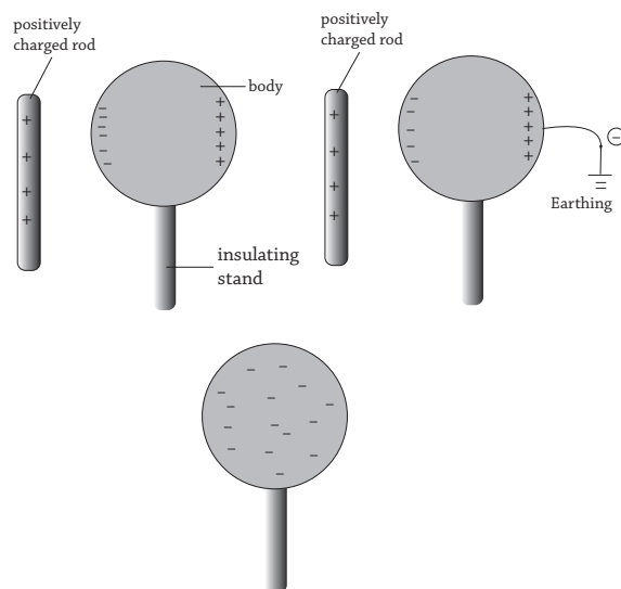
Fig. 16.5: Charging negatively by induction Bring a positively charged rod near a body (metal sphere) on an insulating stand. Negative charges are attracted and positive charges are repelled to the side remote to the charged rod.
