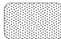
Fig 4.1 : Molecules in a solid
