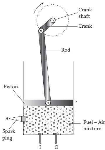
Fig 7.2 : Charging or induction
