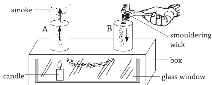
Fig 14.10 : Convectional current in gases
