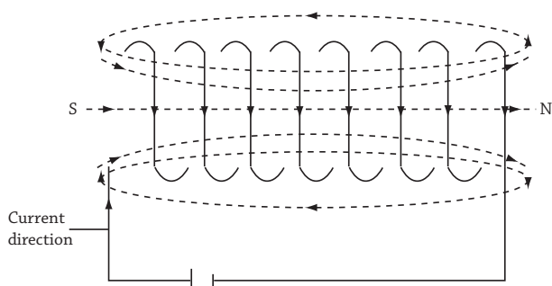
Fig 20.3 : Magnetic field on a solenoid
