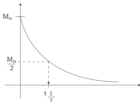
Fig 22.4 : A decay curve
