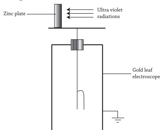
Fig 22.6 : Detecting charges in UV radiation
