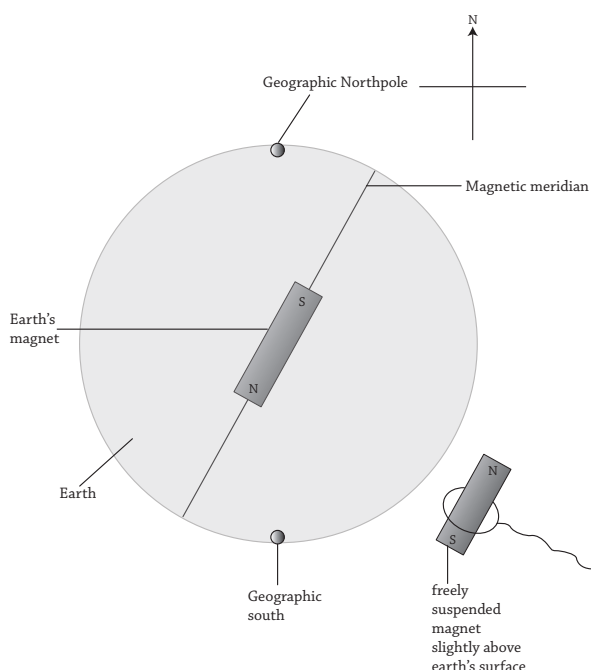
Fig 19.18 : Suspension of bar magnet
