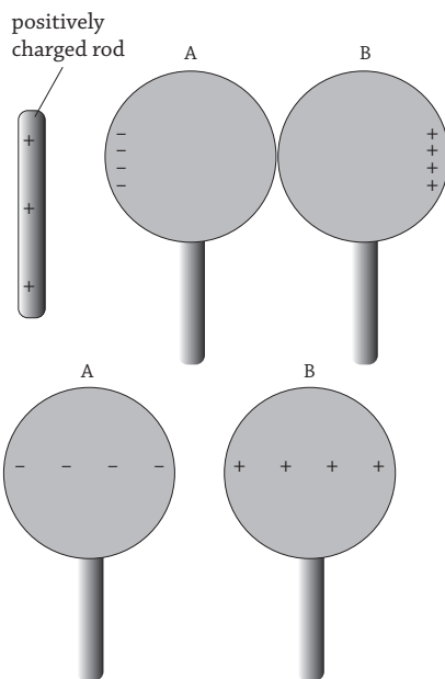
Fig 16.6 : Charging by induction
