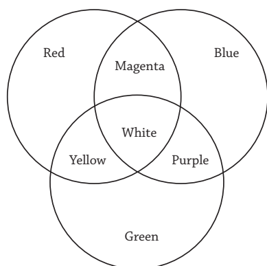
Fig 12.17 : A Colour wheel
