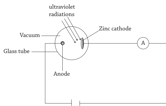
Fig 22.5 : Photoelectric emission
