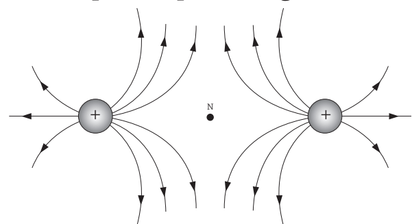
Fig 16.19 : Electric field on two positive charges
