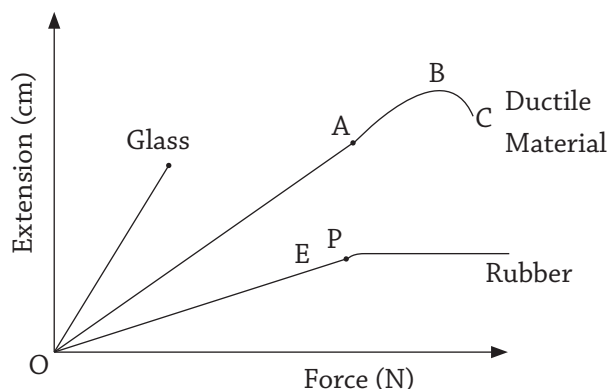
Fig 5.8 : A graph of extension verses force
