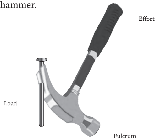
(a) A hammer in use
