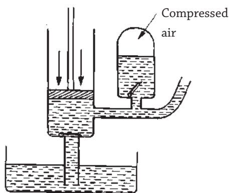
Fig. 8.12 : A force pump
