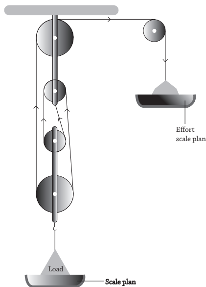
Fig 10.14 : Block and tackle pulley
