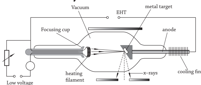
Fig 22.11 : X-ray tube
