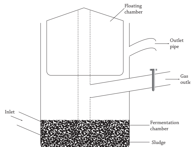
Fig 7.5 : Production of biogas
