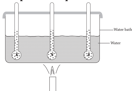
Fig 14.20 : Comparing rates of expansion in liquids.
