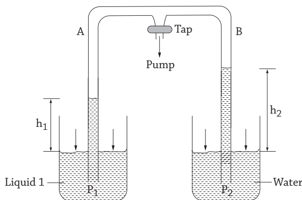
Fig 8.3 : Inverted U-tube
