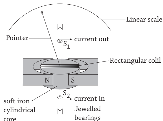
Fig 20.13 : A moving coil galvanometer
