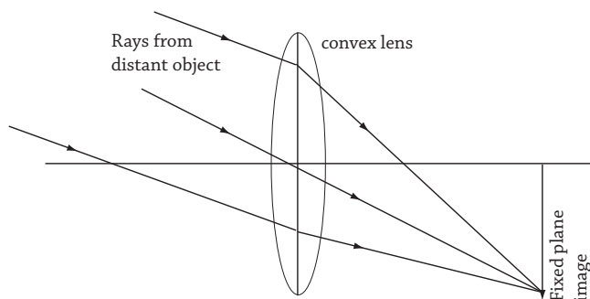
Fig 12.25 : Formation of image on a convex lens
