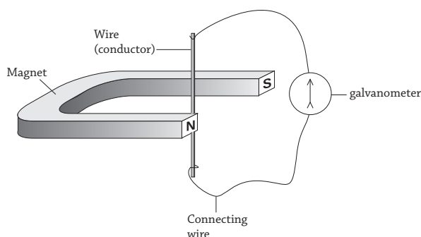
Fig 21.2 : Electromagnetic induction
