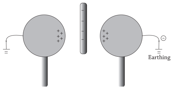
Fig 16.7 (b) : Earthing
