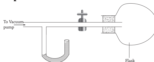
Fig 6.9 : Determining density of air
