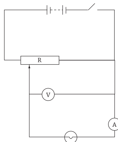
Fig 17.2 : Correct diagram electric circuit
