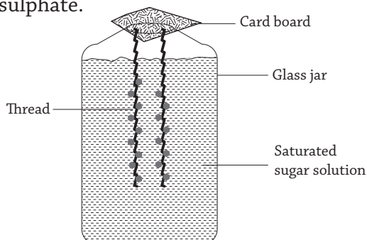
Fig 4.12 : Growing crystals
