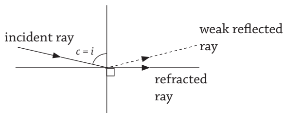
Fig 12.7 : Critical angle
