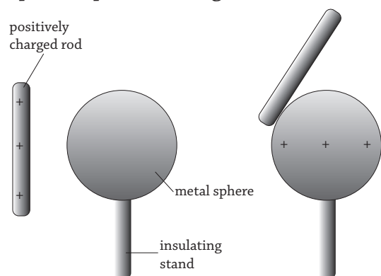
Fig 16.8 : Charging by contact
