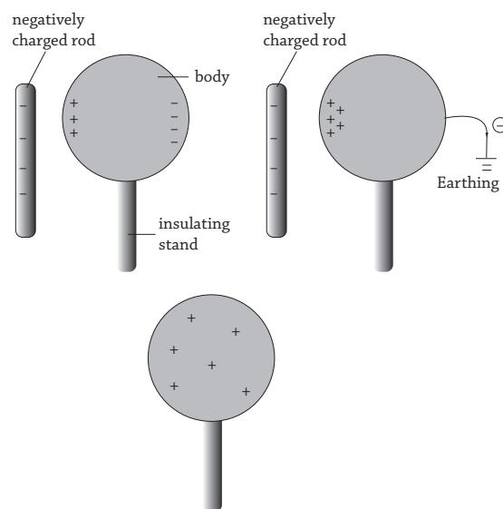
Fig 16.4 : Charging positively by induction Bring a negatively charged rod near a body (metal sphere), on an insulating stand. Positive charges are attracted and negative charges are repelled to the side remote to the charged rod.
