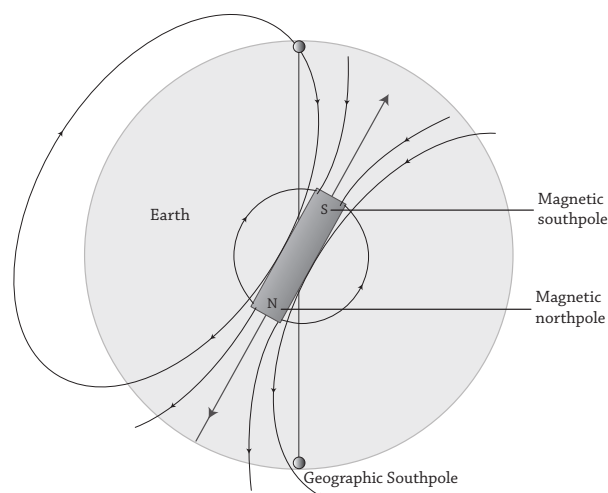
Fig 19.19 : Magnetic field lines
