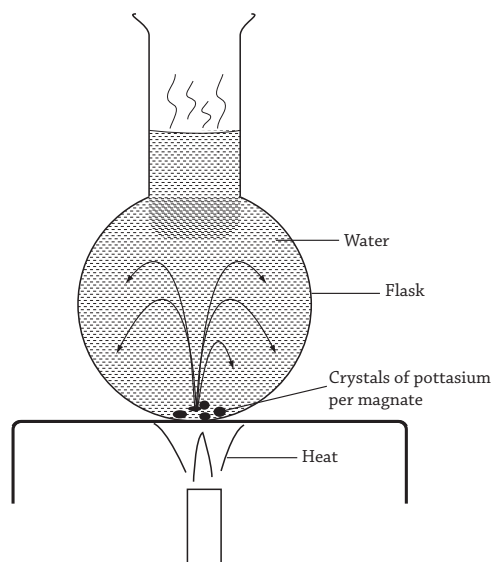
Fig 14.9 Convectional currents in liquids
