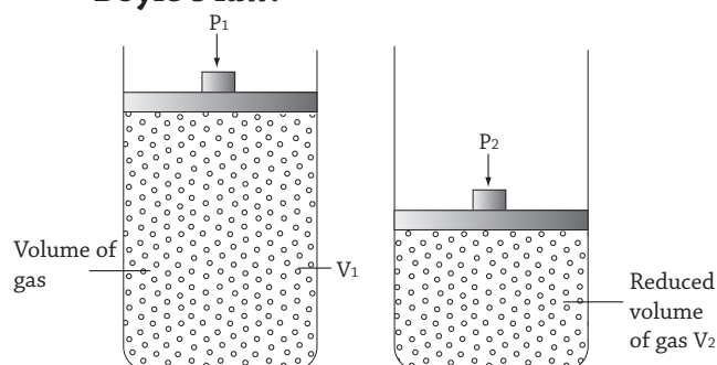
Fig 15.4 : Boyle's law in terms of kinetic theory
