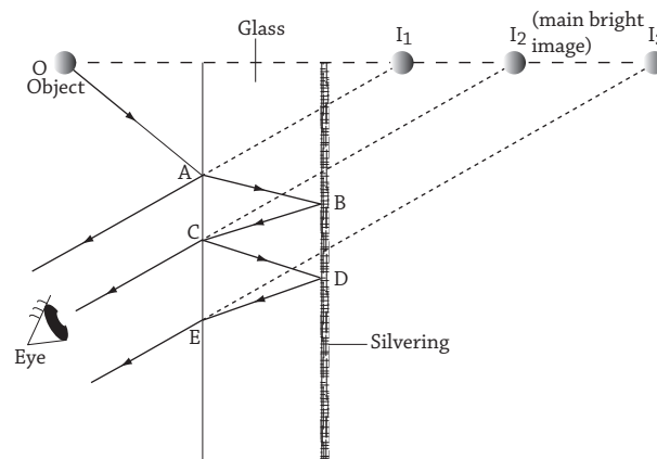
Fig 12.10 : Multiple image due to total internal reflection
