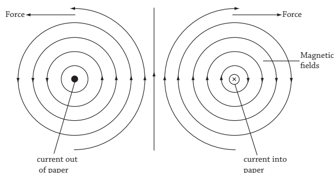
Fig 20.5 : Magnetic fields due to current flowing in opposite direction
