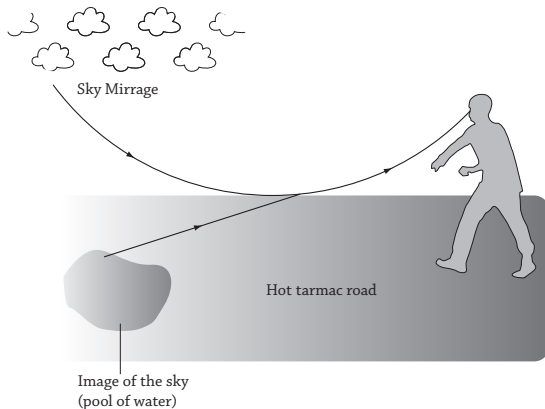
Fig 12.11 Mirages on tarmac road
