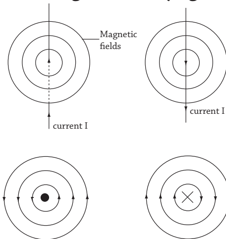
Fig 20.1 : Magnetic field on a straight conductor
