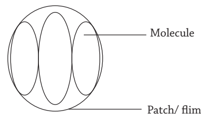
Fig 4.11 : An oil path
