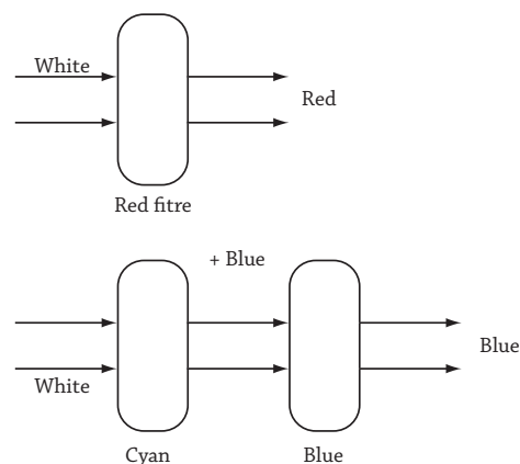
Fig 12.18 : A Colour filters
