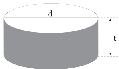
Fig 4.10 : An oil enlarged path
