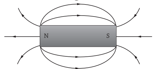
Fig 19.5 : Magnetic field on a bar magnet
