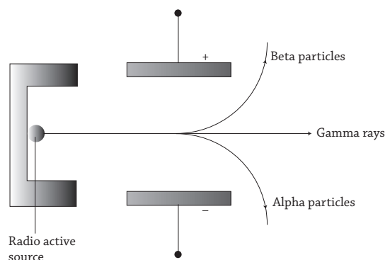
Fig 22.2 : Particles in electric field
