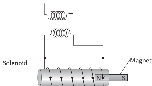
Fig 19.4 : Demagnetising a magnet by electronic method
