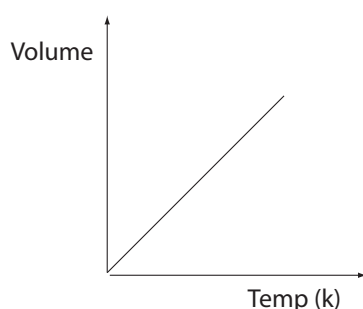
Fig 15.9 : Volume against Temperature Kelvin
