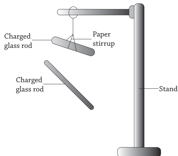
Fig 16.2 : Test of charges
