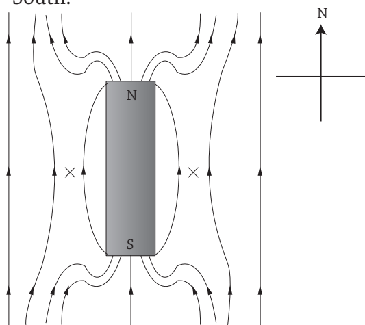
Fig 19.21 : A bar magnet in North – South Direction
