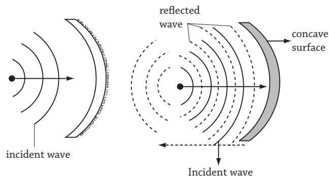
Fig 13.7 (a) : Reflection on concave surface
