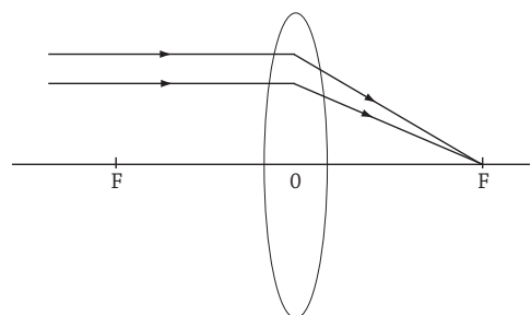
Fig 12.22 : A principal focus of convex lens
