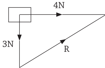
Fig 2.3 (a) resolution of forces
