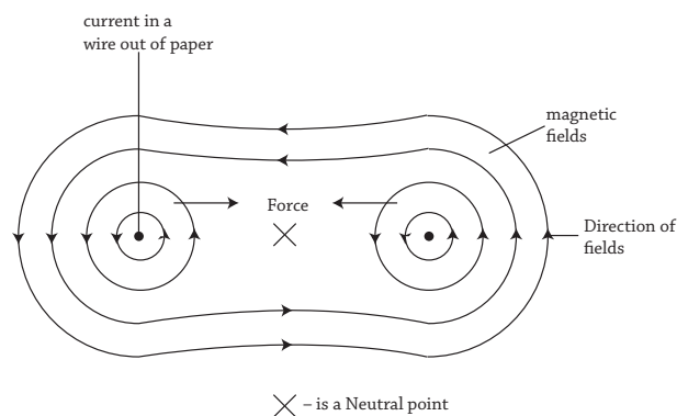
Fig 20.4 : Magnetic fields due to parallel conductors
