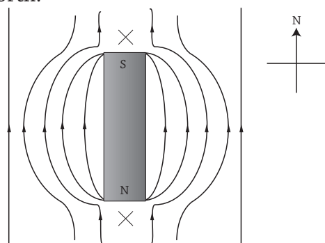
Fig 19.22 : A bar magnet in South – North Direction
