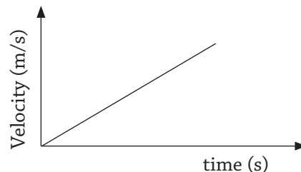
Fig 11.14 : Velocity time graph showing acceleration due to gravity.
