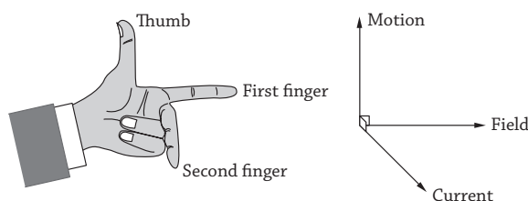
Fig 21.1 : Fleming's right hand rule
