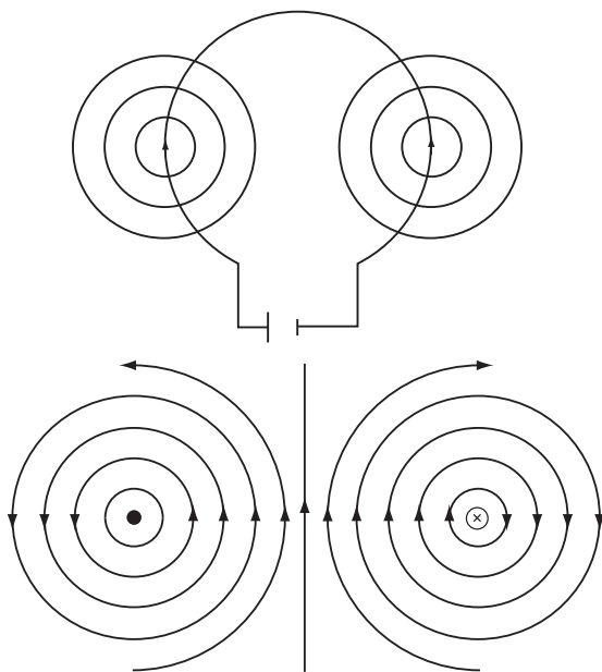
Fig 20.2 : Magnetic field on circular coil
