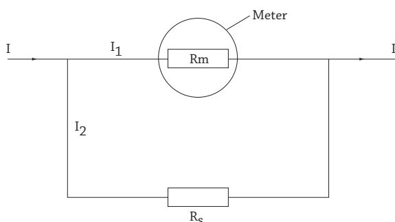
Fig 18.14 : Calibration of resistor
