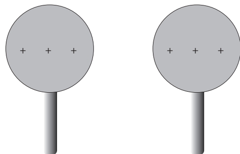
Fig 16.7 (c) : Positively charged rod
