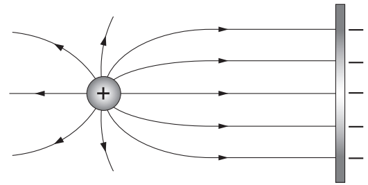
Fig 16.23 : Electric field of point and charges plates
