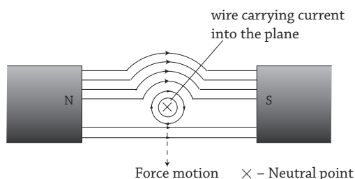
Fig 20.10 : Effect of magnetic field current carrying wire
