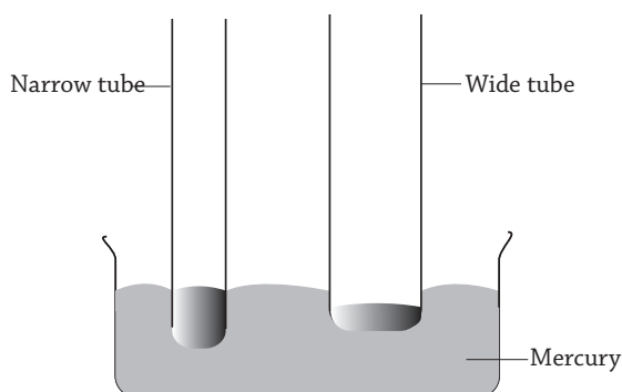
Fig 4.9 : Capillarity in mercury
