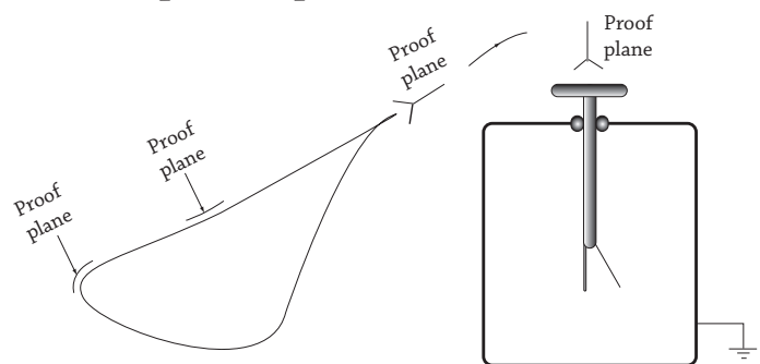
Fig 16.14 : Pear shaped conductor
