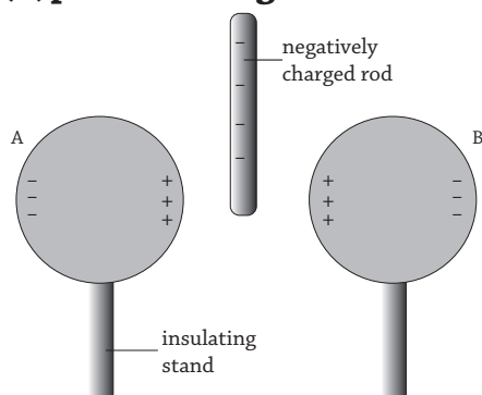
Fig 16.7 (a) : Inserting charged rod between spheres
