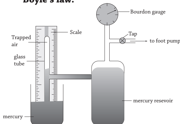
Fig 15.1 : Verifying Boyle's law
