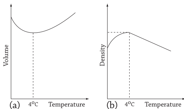
Fig 14.21 : Anomalous expansion of water
