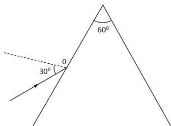
Fig 12.12 (a) : A glass prism refracting monochromatic light
