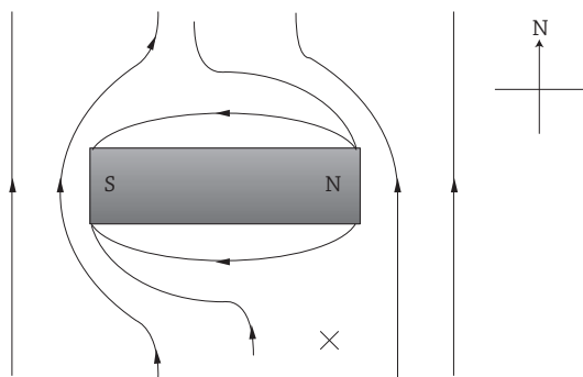
Fig 19.20 : A magnet in West – East direction
