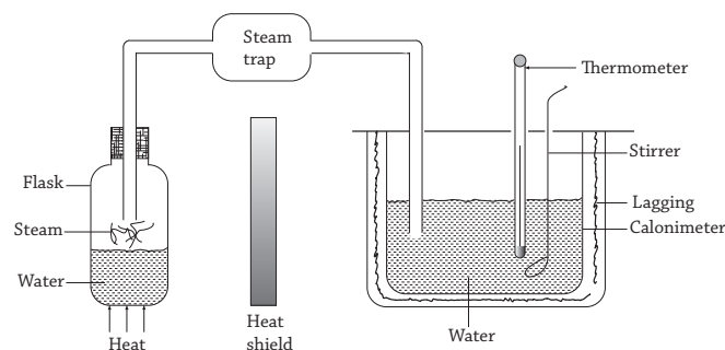
Fig 15.16 : Determining specific latent heat of vapourisation
