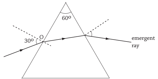
Fig 12.12 (b) : Refraction on a glass prism
