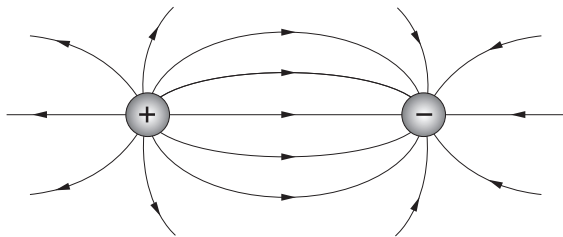
Fig 16.20 : Electric field on opposite plate
