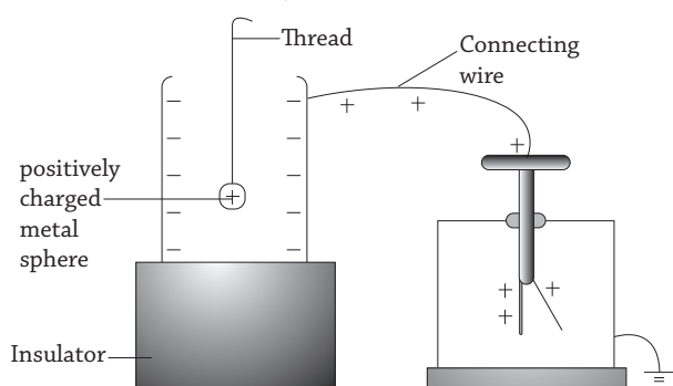
Fig 16.15 : Ice pail experiment
