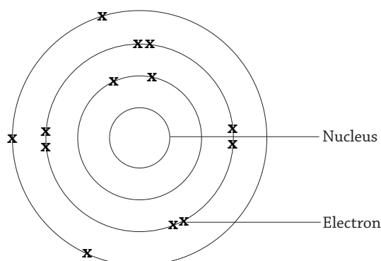
Fig 16.1 : Structure of an atom
