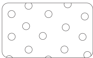
Fig 4.3 : Molecules in gases
