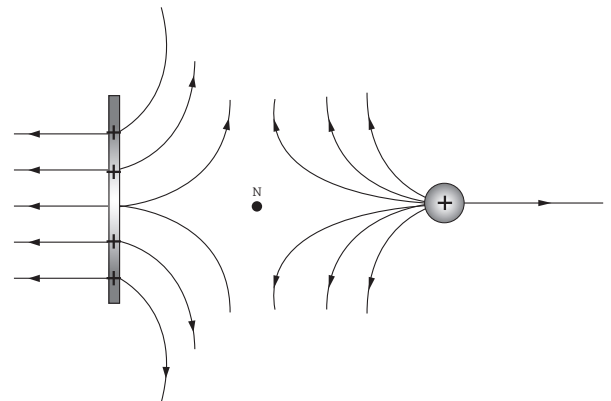
Fig 16.24 : Electric field on similar
