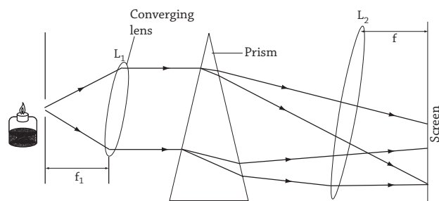
Fig 12.16 : Production of spectrum
