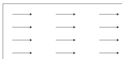
Fig 19.11 (c) : Magnetised material
