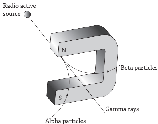
Fig 22.3 : Particles in a magnetic field
