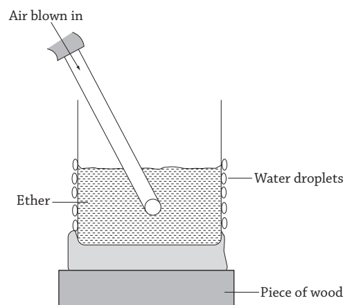
Fig 15.22 : Cooling effect of evaporation
