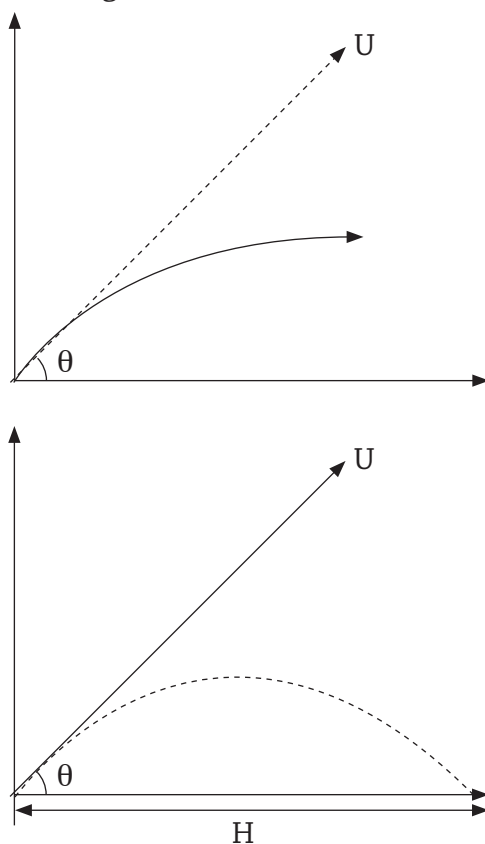
Fig 11.17 : Projectile motion
