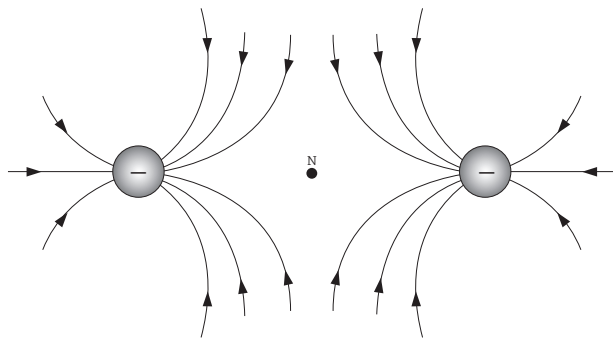
Fig 16.19 : Electric field of two negative charges
