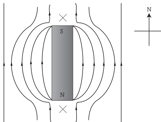
Fig 19.23 : Magnetic field pattern near a bar magnet
