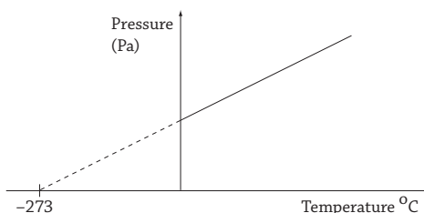
Fig 15.11 : A graph of pressure against temperature
