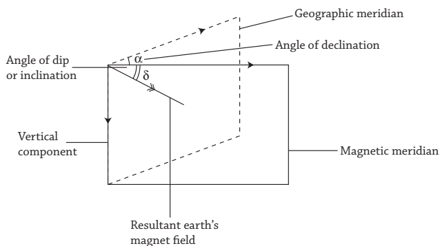
Fig 19.17 : Earth's magnetic field
