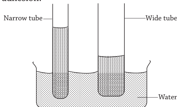
Fig 4.8 : Capillarity in water
