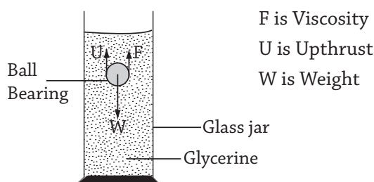
Fig 2.7 : Motion of body in fluid
