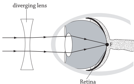
Fig 12.40 : Correction of short-sightedness
