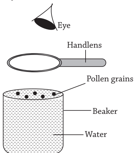
Fig 4.5 Pollen grains on water
