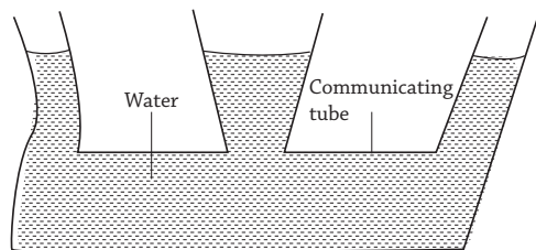
Fig 8.5 : Water takes the shape of container
