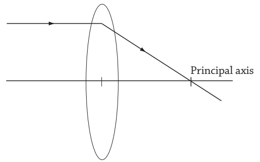
Fig 12.20 : A Convex lens
