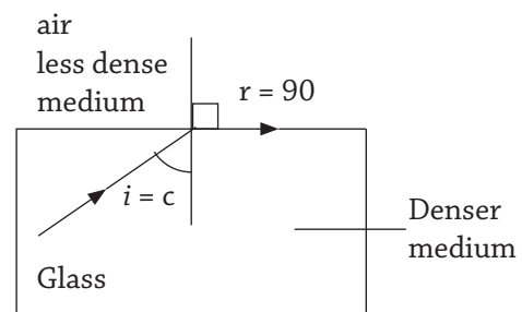
Fig 12.13 : A glass block
