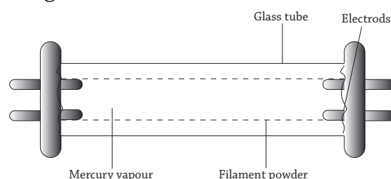
Fig 18.19 : A florescent tube
