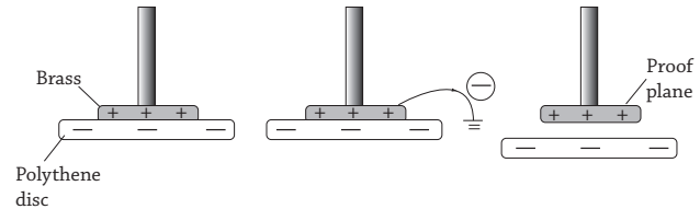
Fig 16.13 : Charging electrophorons
