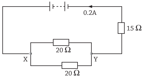
Fig 18.6 : An electric circuit
