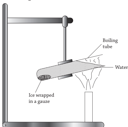
Fig 14.7 : Determination of poor thermal conductivity of water
