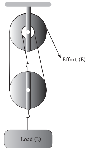
Fig 10.19 : A pulley system
