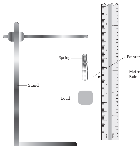
Fig 5.6 : Verification of Hook's Law
