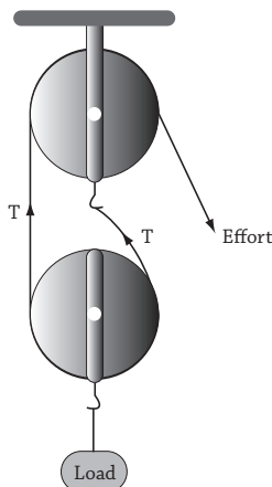
Fig 10.10 : A fixed and moveable pulley
