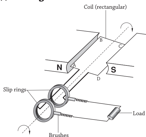
Fig 21.4 (a) : An alternating current (a.c) generator
