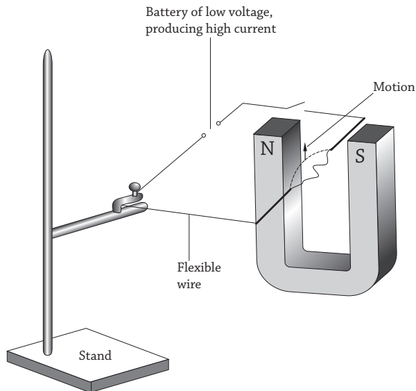
Fig 20.9 : Demonstrating motor effect
