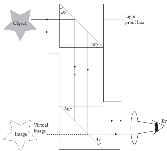
Fig 12.9 : A prism periscope
