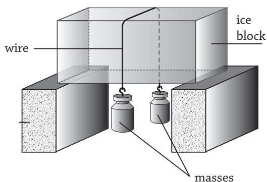
Fig 15.17 : Effect of pressure on melting point
