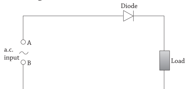
Fig 21.7 : An a.c. circuit of half-wave rectification
