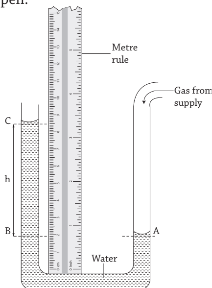
Fig 8.9 : A U-tube manometer
