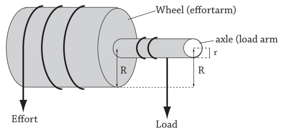
Fig 10.4 : Wheel and axle
