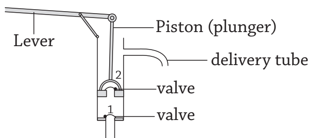
Fig 8.13 : A lift pump
