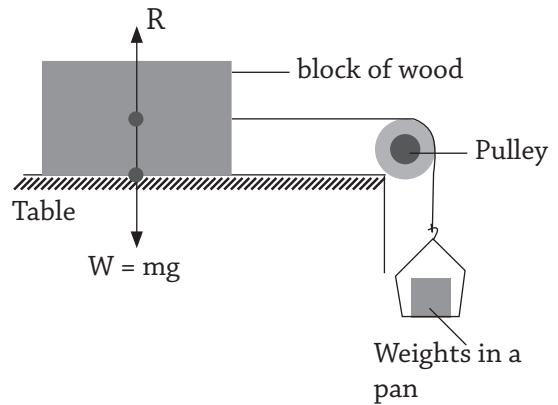
Fig 2.6 : Determining the coefficient of static friction
