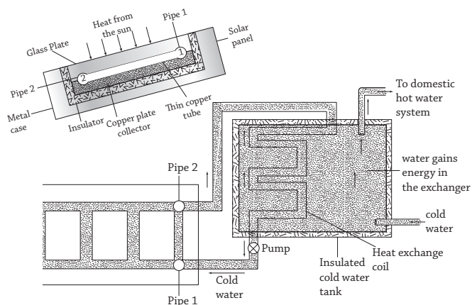
Fig 14.14 : Solar heating system
