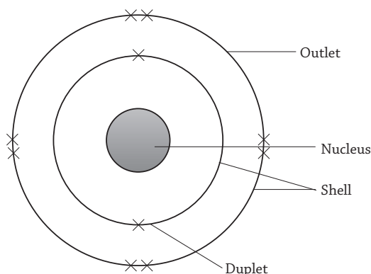
Fig 21.1 : Structure of an atom
