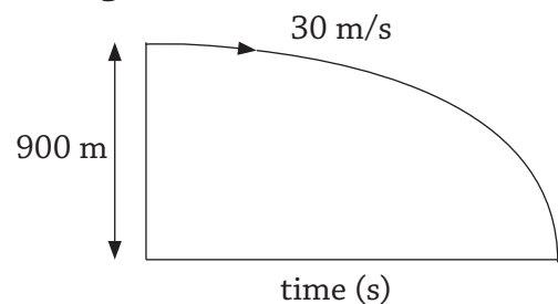
Fig 11.18 : Projection motion
