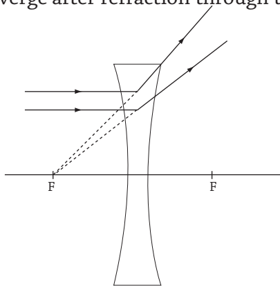
Fig 12.23 : Principal focus of concave lens
