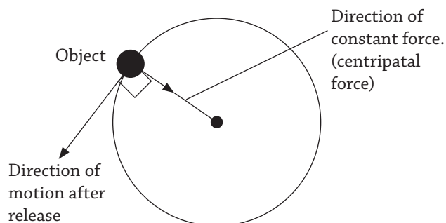
Fig. 11.16 : Circular motion
