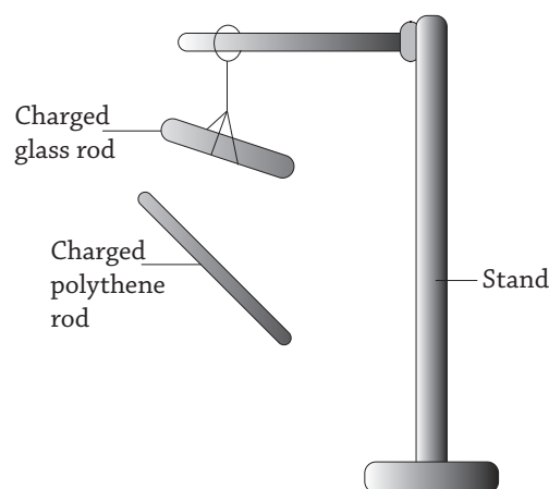
Fig 16.3 : Test of charges
