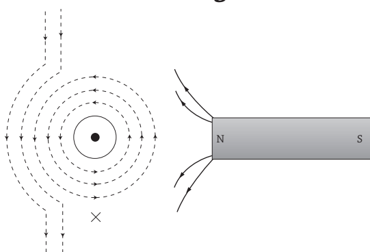
Fig 19.9 : Magnetic field due to electric current
