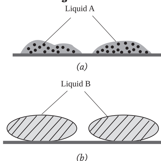
Fig 4.7 : Molecules of liquids
