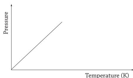
Fig 15.12 : A graph of pressure against temperature (K)
