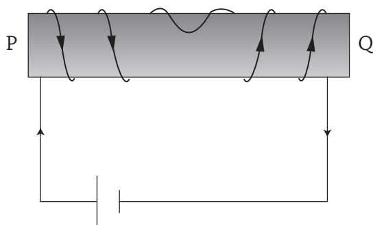
Fig 19.12 (b) : Identifying poles
