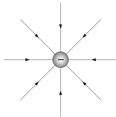
Fig 16.18 : Electric field on negative charge
