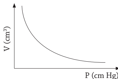
Fig 15.3 : A graph of V against P
