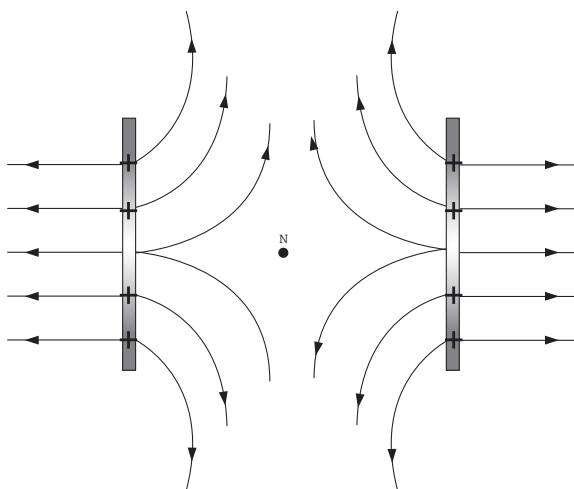
Fig 16.22 : Electric field on similar plates
