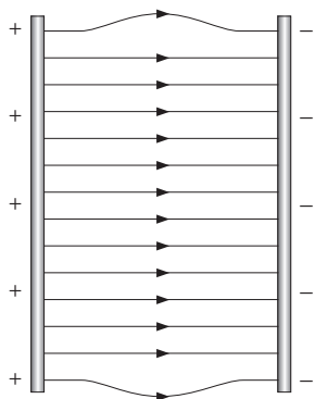
Fig 16.21 : Electric field on opposite plate
