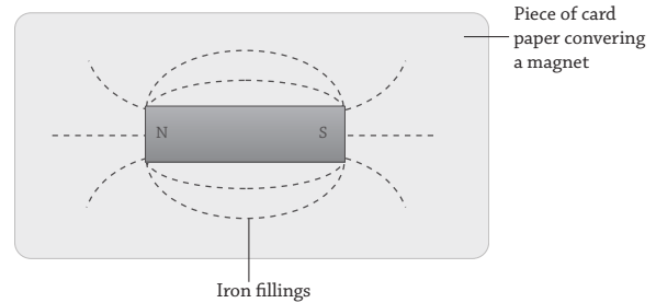
Fig 19.16 : Magnetic field lines
