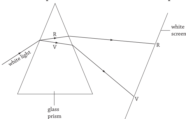
Fig 12.19 : Colour spectrum
