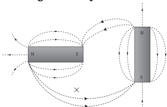
Fig 19.10 (b) : magnetic field due to two magnets
