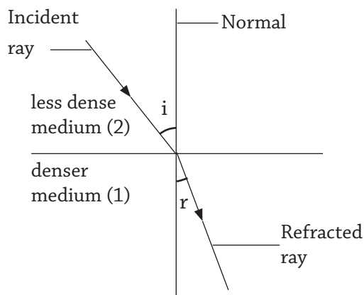
Fig 12.1 (a) : Refraction of light
