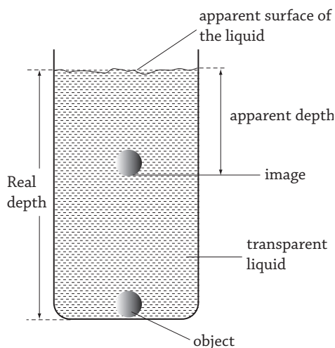
Fig 12.5 : Real and apparent depth
