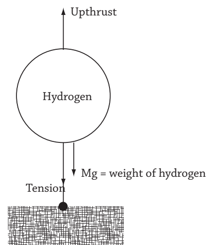
Fig 9.6 : Force acting on suspended balloon
