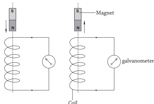
Fig 21.3 : Demonstrating Lenz's law
