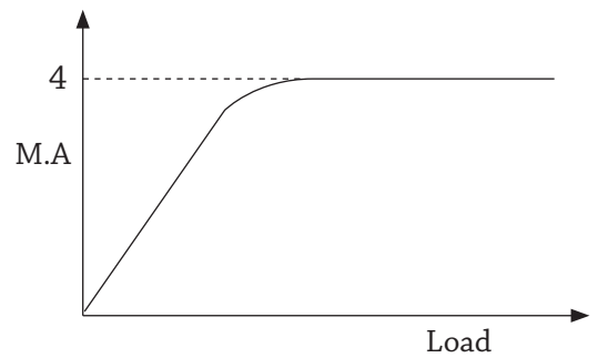
Fig 10.15 : A graph of M.A against load
