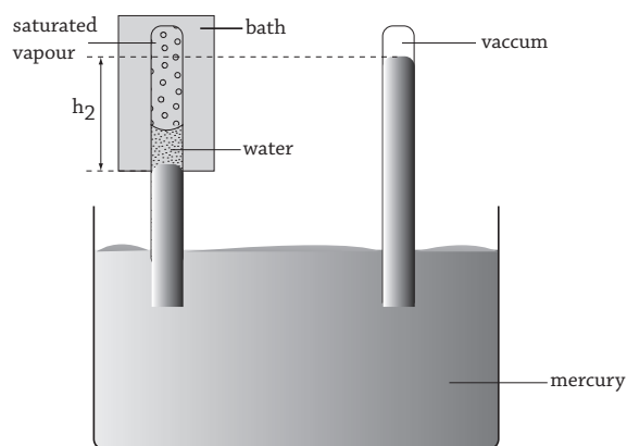
Fig 15.21 : Measuring the vapour pressure of water
