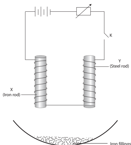
Fig 19.13 : Magnetising soft iron core
