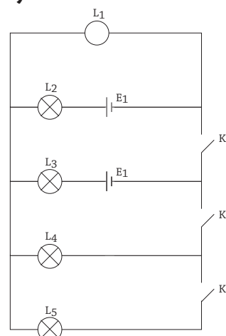
Fig.17.5 : Cells and bulbs in parallel
