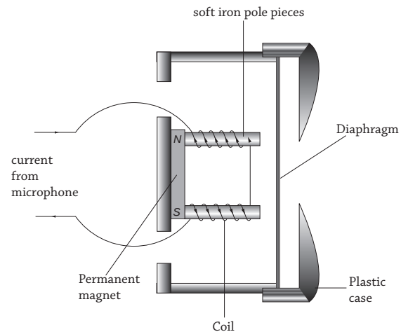
Fig 20.8 : Telephone receiver
