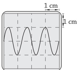
Fig 22.10 : A Sinusoidal wave on CRO
