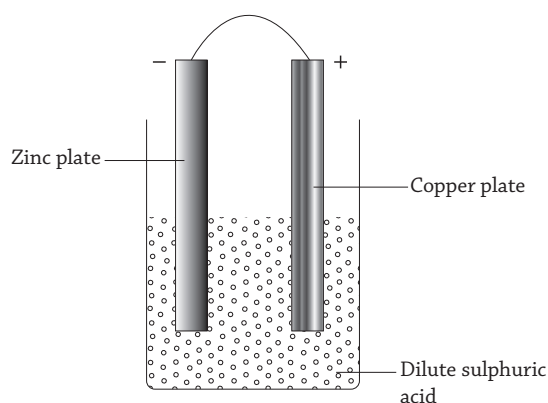
Fig 17.6 : Primary cell
