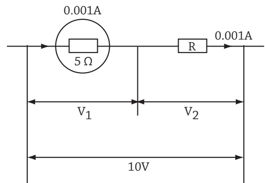
Fig 18.8 : Calibration of meters
