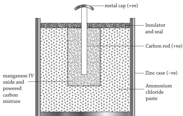
Fig 17.7 : A dry cell
