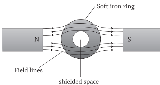
Fig 19.14 : Magnetic shielding
