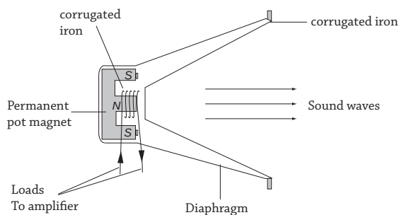
Fig 20.7 : A microphone
