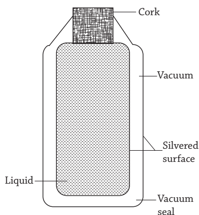
Fig 14.12 : A vacuum flask
