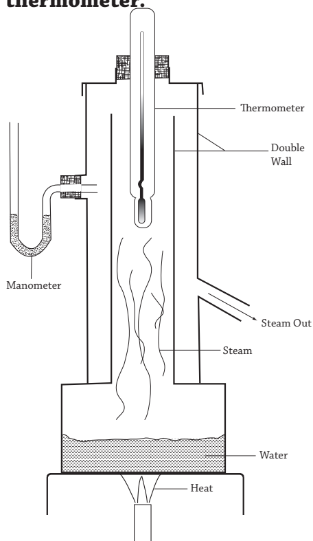
Fig 14.5 : Determination of upper fixed point. (Hypsometer)
