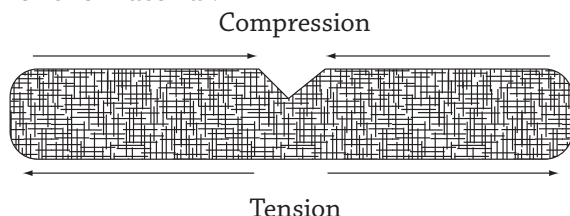
Fig 5.5 : Norch effect
