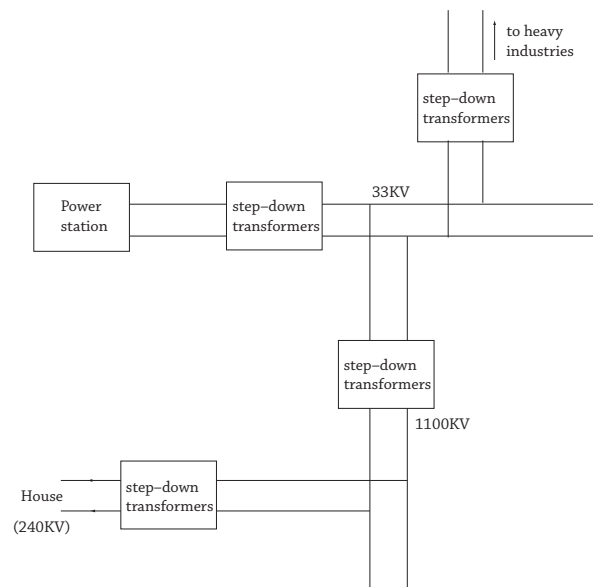
Fig 18.20 : Power transmission process
