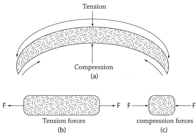
Fig 5.2 : Objects under tension and compression
