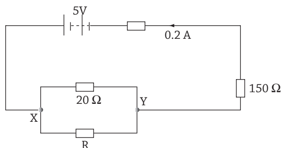
Fig 18.5 : Electric circuit
