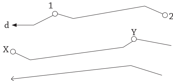
Fig 18.21 : Two way switch
