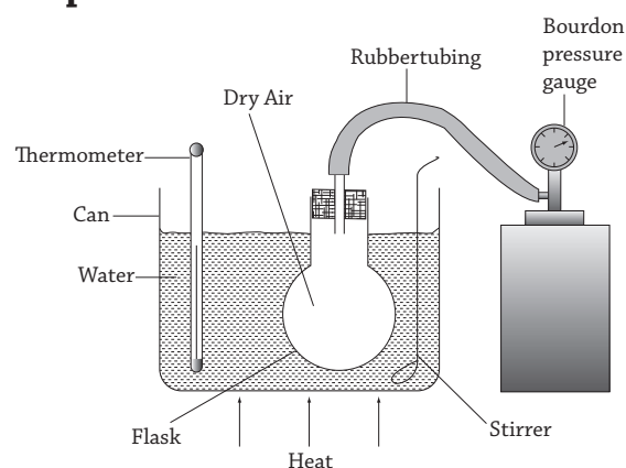
Fig 15.10 : Verifying pressure law
