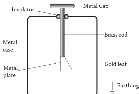
Fig 16.9 : A gold leaf electroscope
