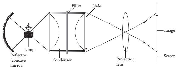
Fig 12.44 : A slide projector
