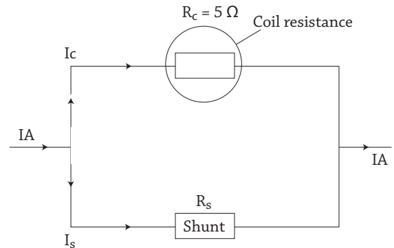
Fig 21.10 : Converting a moving coil meter scales
